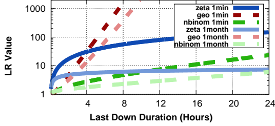
Fig. 11. Comparison of LR values, between zeta, geometric and negative binomial distribution for the value t_d^i set to one minute and one month. Considering each t_d^i value separately, negative binomial distribution is the better choice.
